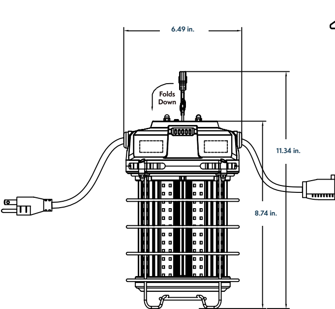
1006 100W Dimensions:
